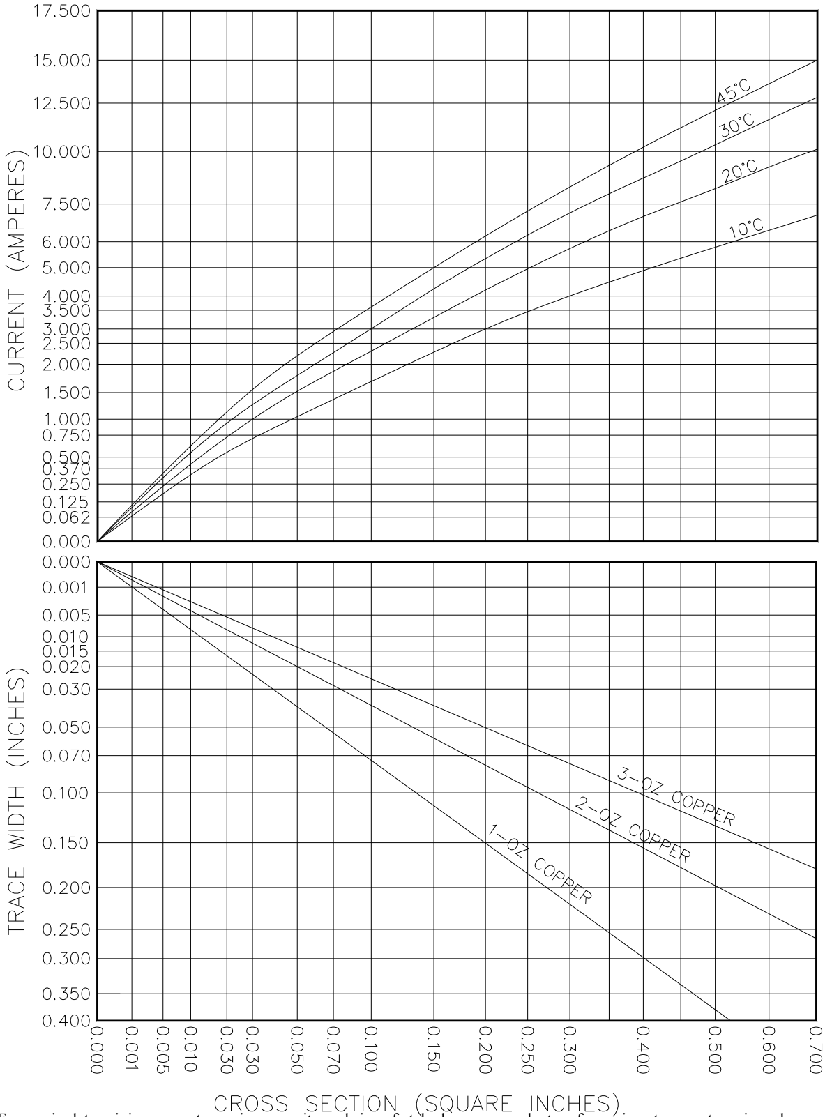
For use in determining current carrying capacity and size of etched copper conductors for various temperature rises above ambient
